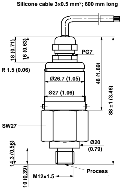
Fig. 7: Piston pressure switch type KD1-...-K2
