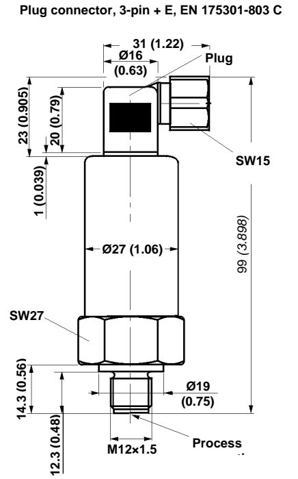
Fig. 10: Piston/diaphragm pressure switch type KLK/KLM-...-S1
