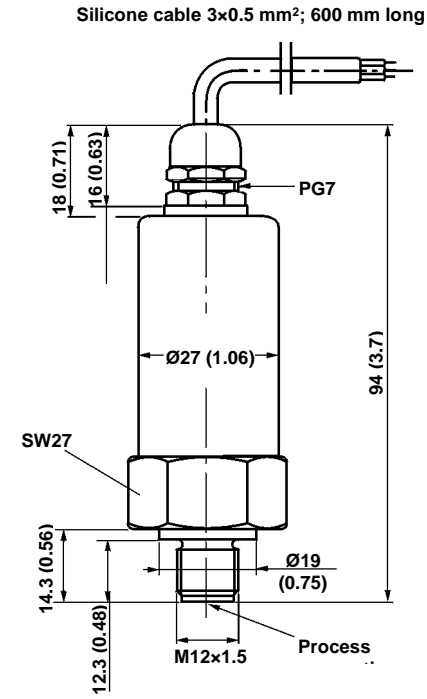
Fig. 9: Piston/diaphragm pressure switch type KLK/KLM-...-K2
