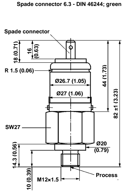
Fig. 8: Piston pressure switch type KD1-...-A1
